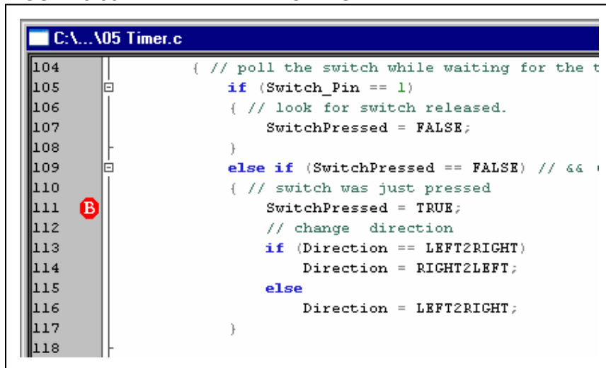
FIGURE 3-30: BREAKPOINT SET
