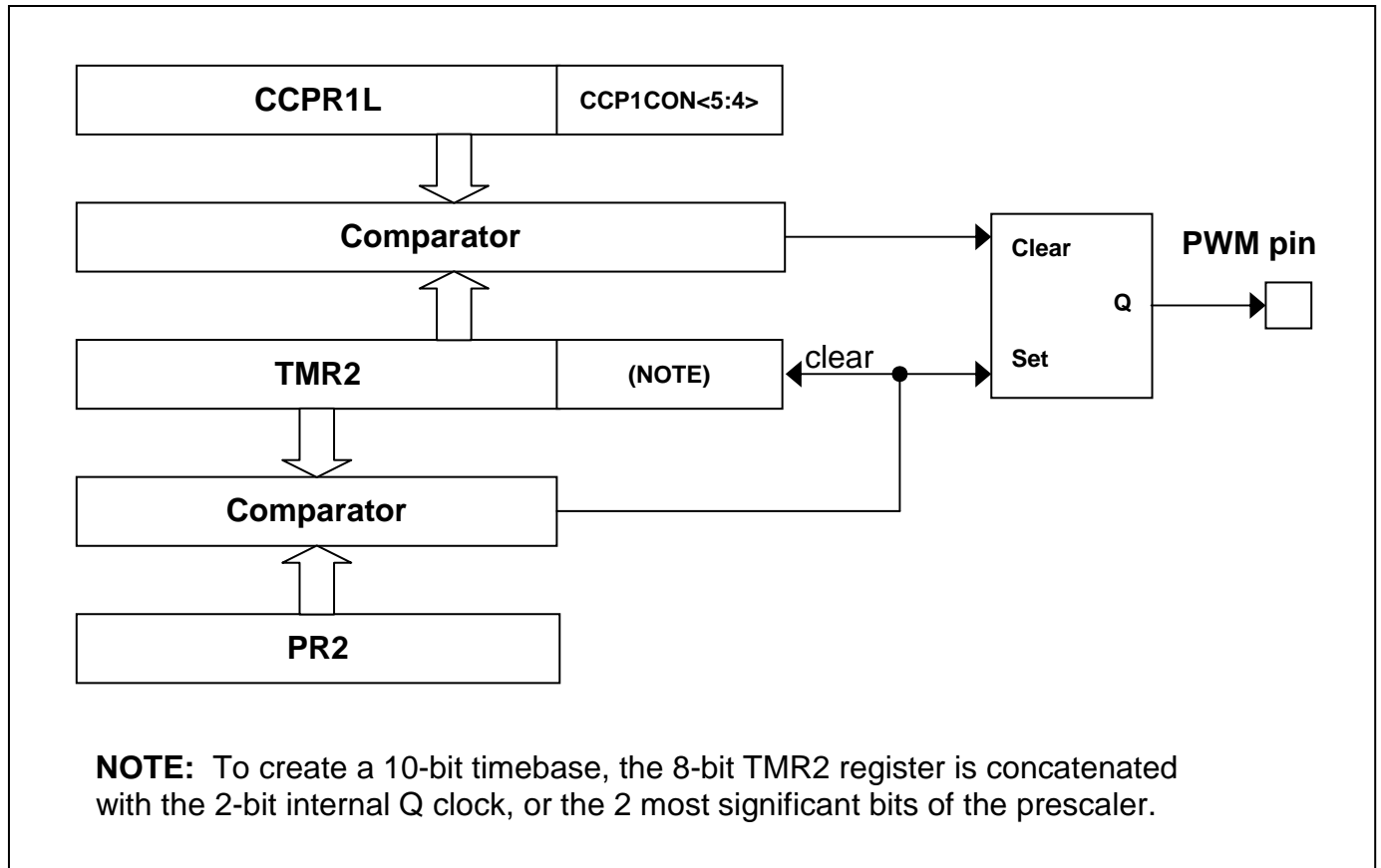
FIGURE 3-57: SIMPLIFIED PWM BLOCK DIAGRAM
