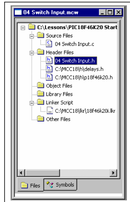
FIGURE 3-20 HEADER FILE
