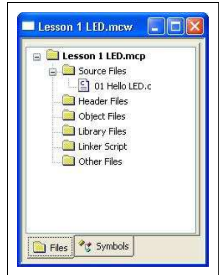
FIGURE 3-5: PROJECT WINDOW
