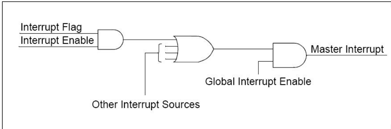
FIGURE 3-37: SIMPLIFIED INTERRUPT LOGIC
