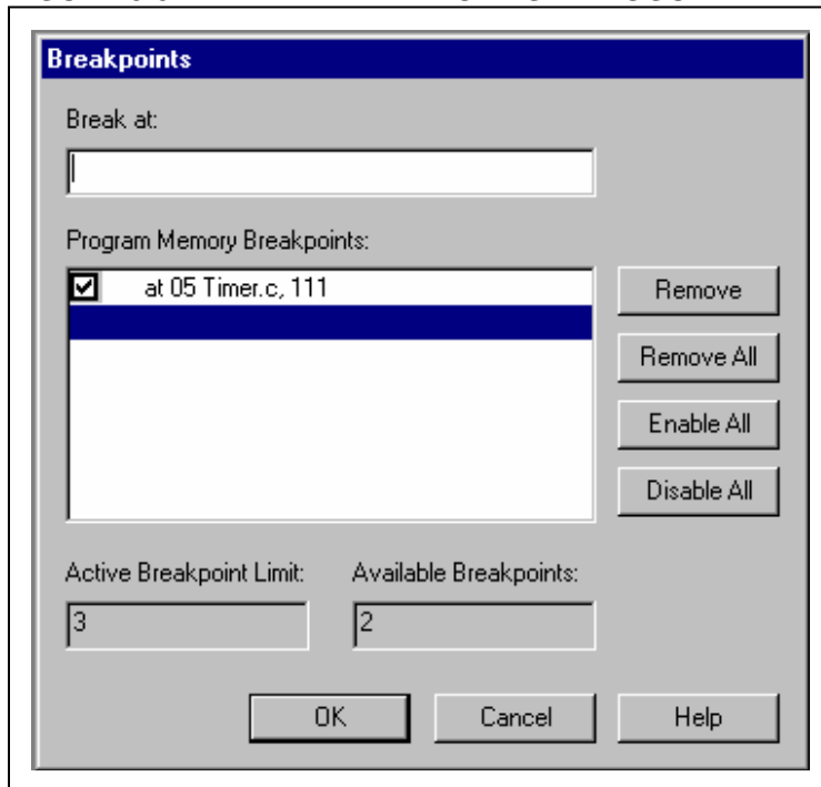
FIGURE 3-32: BREAKPOINTS DIALOGUE
