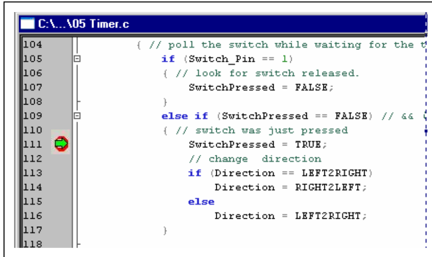
FIGURE 3-31: BREAKPOINT HALT
