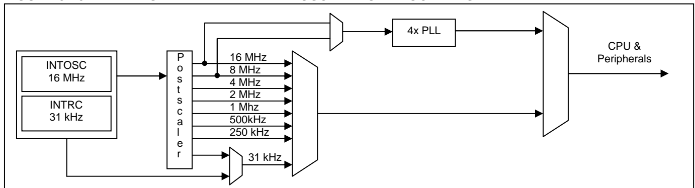
FIGURE 3-43: SIMPLIFIED INTERNAL OSCILLATOR BLOCK DIAGRAM
